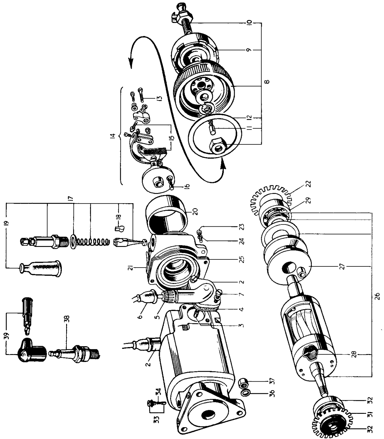
FIG. 35 MAGNETO WITH MANUAL CONTROL
