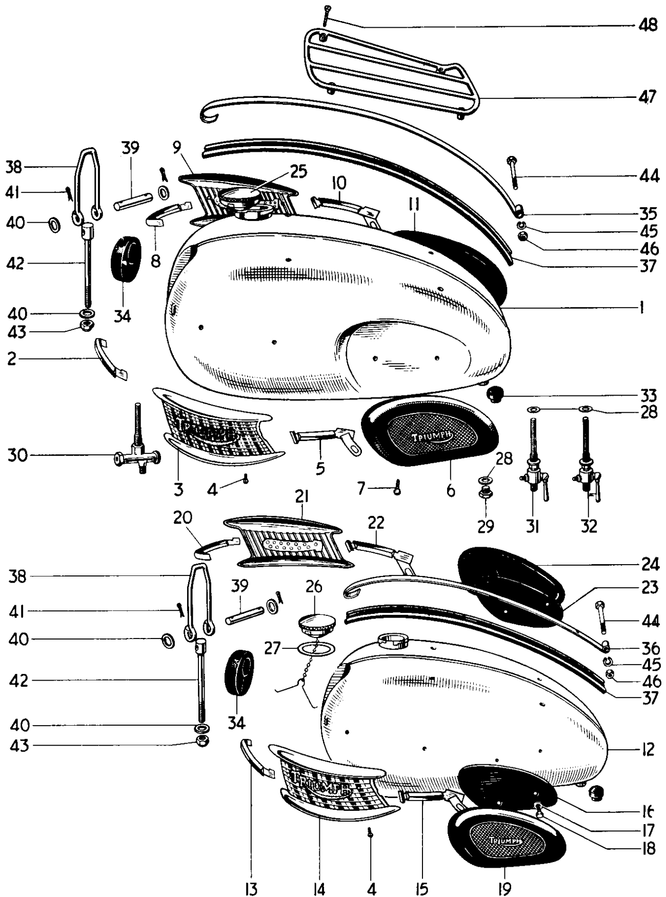
FIG. 23 PETROL TANKS
