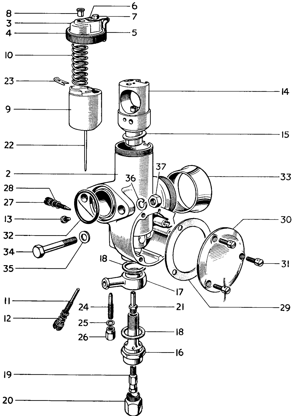
FIG. 32 BONNEVILLE 120 CARBURETTERS
